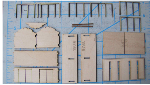
Pieces separated
