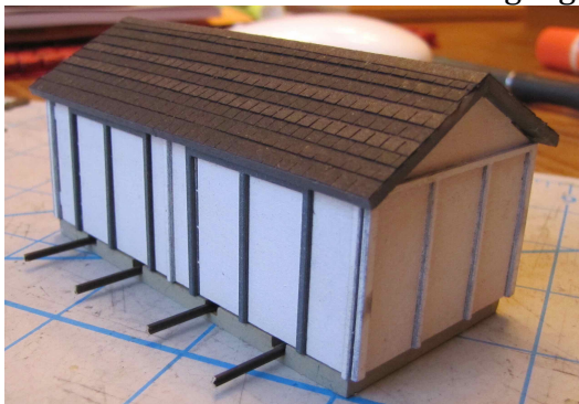
Glue in rails to foundation. Check gauge.
