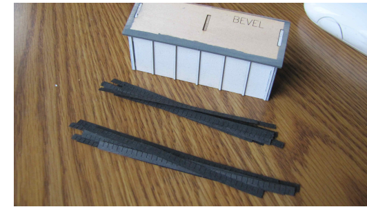
Shingle the roof by gluing on the strips.
