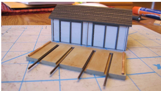
Glue in rails to foundation. Check gauge.
