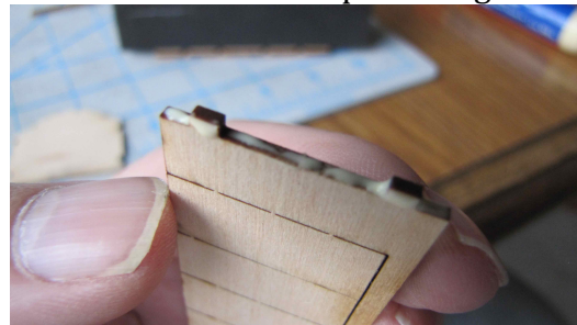
Glue the 4 sides keeping them square.
